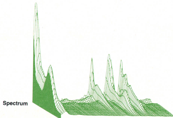
Fig. 3. By repetitive measurements, the HP 1040A generates absorbance data as a function of wavelength and time.
