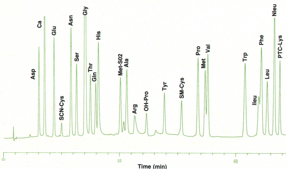
Fig. 1. An HP 1090 chromatogram showing all 25 PTH amino acids separated on a 100 \times 2.1 -mm reversed-phase column.
