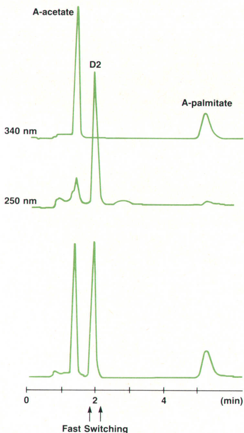
Fig. 7. An autobalance function allows filter changes during a run within two seconds, as shown in the lower chromatogram.
