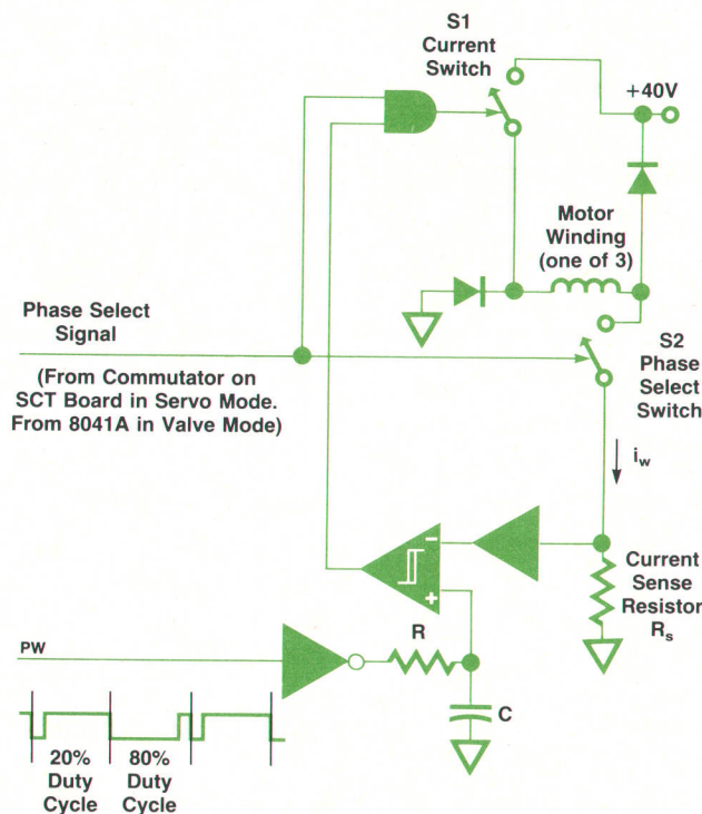
Fig. 13. Output stage of the motor driver is a half-active switched-mode bridge amplifier. The switches S1 and S2 are controlled by the amplifier control logic in Fig. 12.
