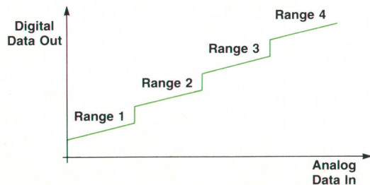
Fig. 15. This nonlinear transfer characteristic of the front-end ADC is corrected by the data acquisition processor (DAP).
