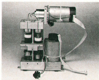
Fig. 3. Metering pump and rotary valve assembly. High-precision sapphire pistons and a high-performance drive system provide accurate volume displacement.
