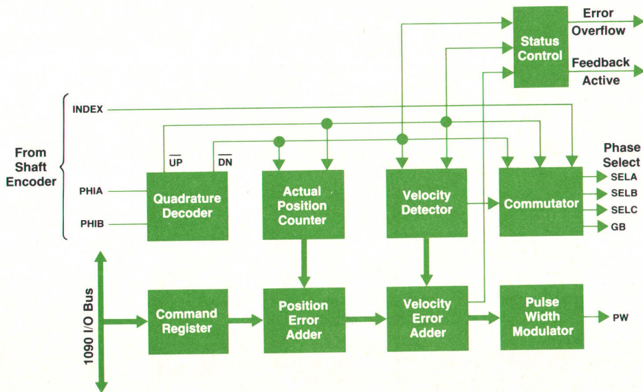
Fig. 10. Solvent delivery system electronic block diagram.
