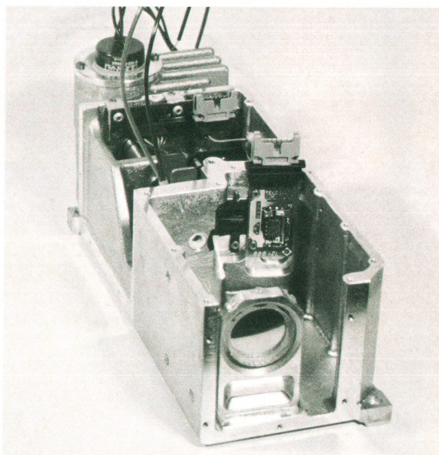
Fig. 13. The optical unit (lighthouse, illumination compartment, spectrometer) is housed in a casting.
