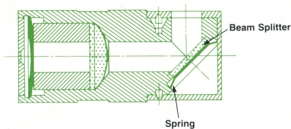
Fig. 5. Lens housing, showing location of micro spring.
