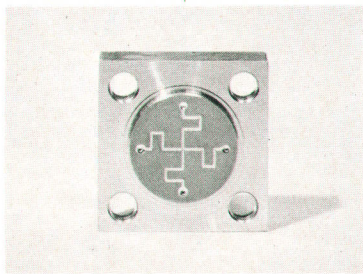
Fig. 6. The low-pressure compliance (LPC) connects the metering pump to the high-pressure pump. The contributions of the three solvent channels are combined in the mixing chamber (photo). The deflection of the diaphragm of the LPC is measured by a strain gauge system mounted on a prestressed spring.
