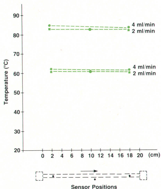
Fig. 2. Temperatures measured in the column 1.5 cm from the inlet and outlet and in air close to the column wall, using the combined solvent-plus-column thermostat. Temperatures for different flow rates and temperature setpoints vary by 1.5°C or less.
