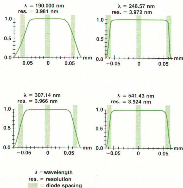
Fig. 9. Intensity distributions of the slit image for pairs of diodes at different points in the diode array, corresponding to different wavelengths.
